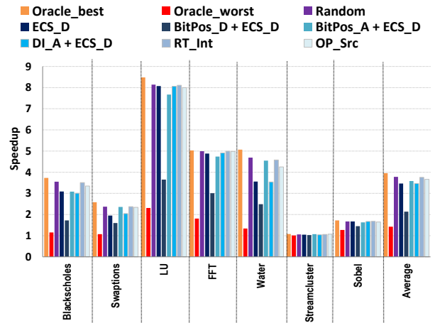
Figure 10. Ref speedup with error-injection prioritization.
